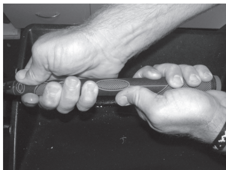
Step 7 - Install Grip. RED 'G' up for right handed golfer, WHITE 'G' up for left handed golfer
